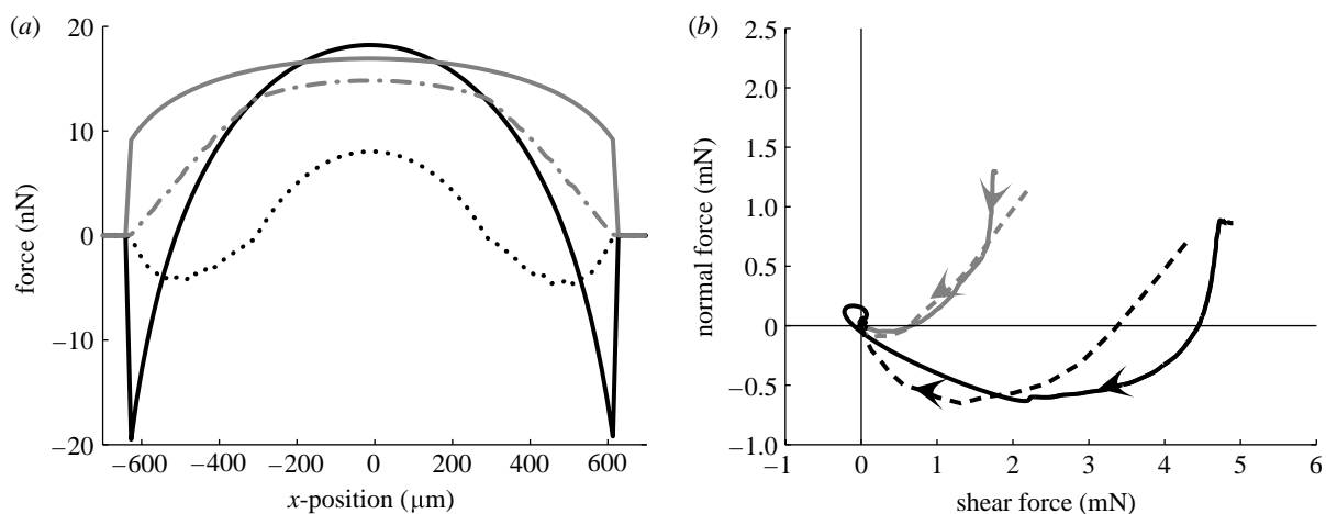
Figure 11. (a) Calculated normal and shear force on fibres under centreline of probe during pull-off for probe indentation 4 \mu\text{m} , and fibres inclined at \theta_0=70^\circ from horizontal. Fibre height variation significantly reduces normal force. Black line, F_n ( l=18.5 \mu\text{m} ); dotted line, F_n ( 17 < l < 20 \mu\text{m} ); grey line, F_t ( l=18.5 \mu\text{m} ); dot-dashed line, F_t ( 17 < l < 20 \mu\text{m} ). (b) Force space plot of predicted normal and shear forces during pull-off for fibres with rest angles of 70^\circ and 85^\circ , and plots of the pull-off portion of the first LDP trial and the 146th trial for a polypropylene fibre array. Grey line, first shear test; black line, 146th shear test; grey dashed line, 85^\circ fibres; black dashed line, 70^\circ fibres.
