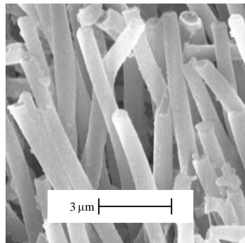
Figure 2. A scanning electron microscope (SEM) image showing shape of tips of synthetic microfibres ( l = 20\text{ }\mu\text{m} and r = 0.3\text{ }\mu\text{m} ).
